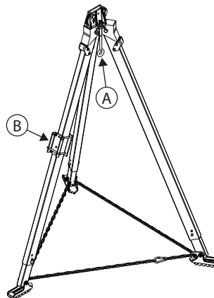
Figure 10 - Tripod Mounting Locations
