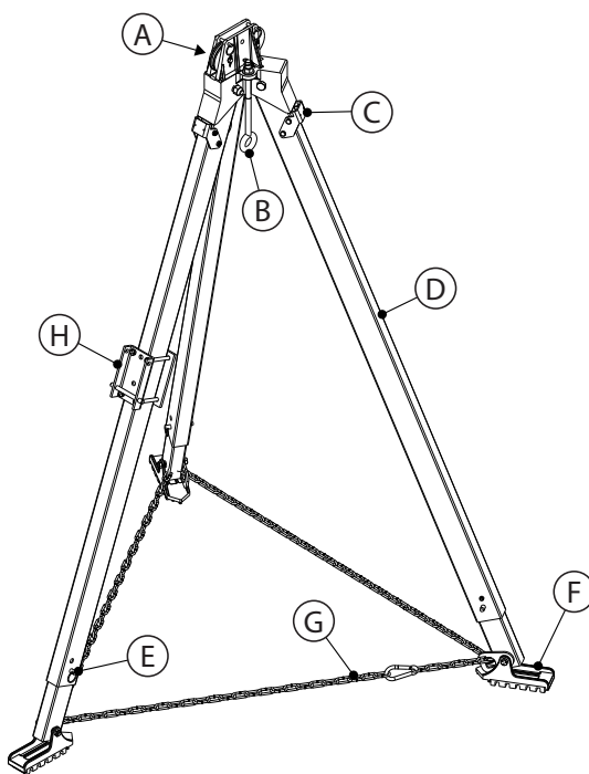
Figure 2 – Composants
