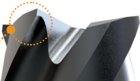
Chip Pocket with large RE (2RE/DC>33%)
