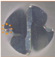
Severe damage to corners
