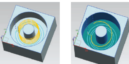
Conventional Helical Milling 7 passes needed VQ4MVM Helical and Ramping Only 1 pass needed
