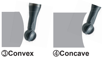
Internal Profile
