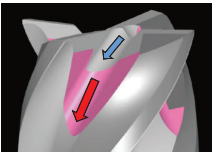
1st Gash 2nd Gash
