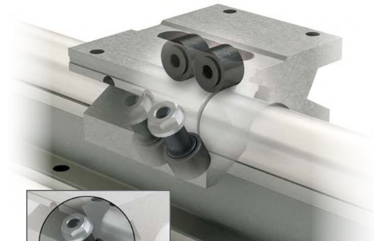
Eccentric bearing adjustment enables fine-tuned adjustments
