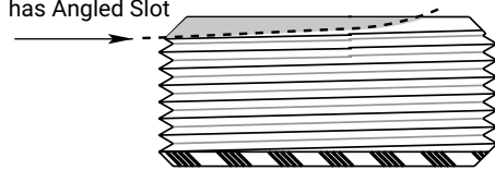
Frelon® Bearing Surface (Approx. 0.025 thick) 3/4 - 20 CLASS #2 Thread
