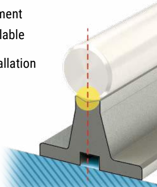
V-block shaped support rail design aligns shaft centerlines simplifying joined rail assemblies
