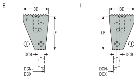
1. Locking screw
