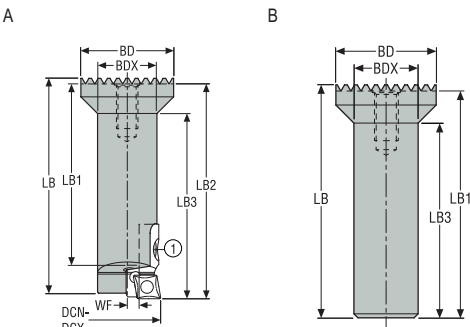
1. Assembly screw
