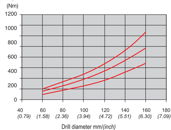
Drilling torque
