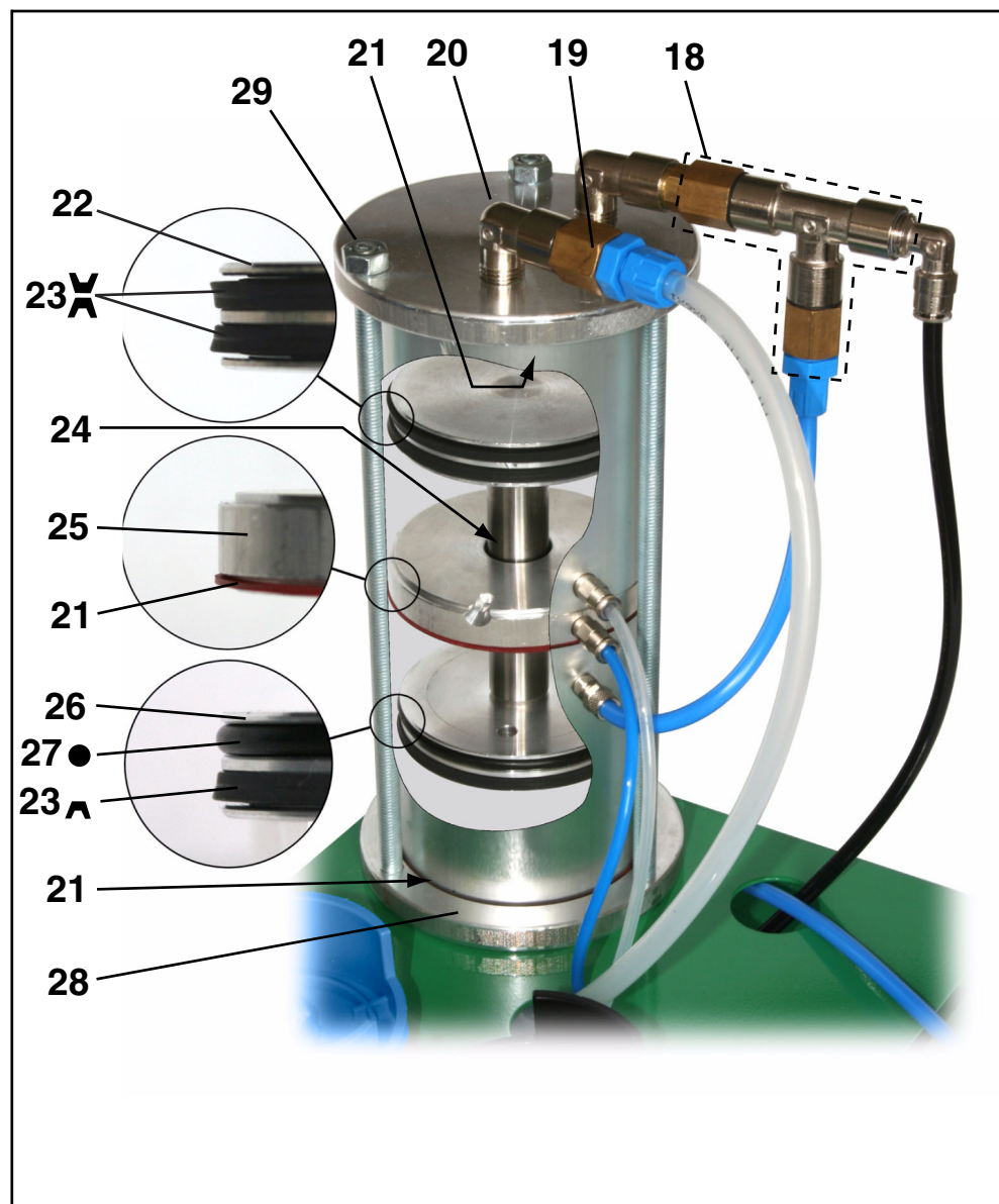
Overview cylinder
